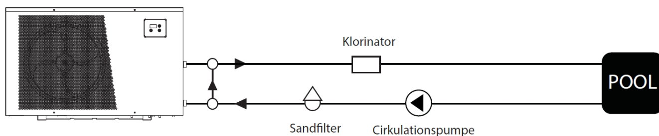
Principskitse for installation
